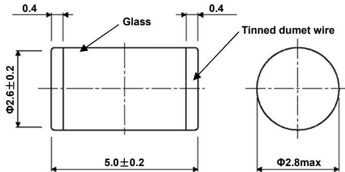
Standard Glass Case JEDEC LL 41
