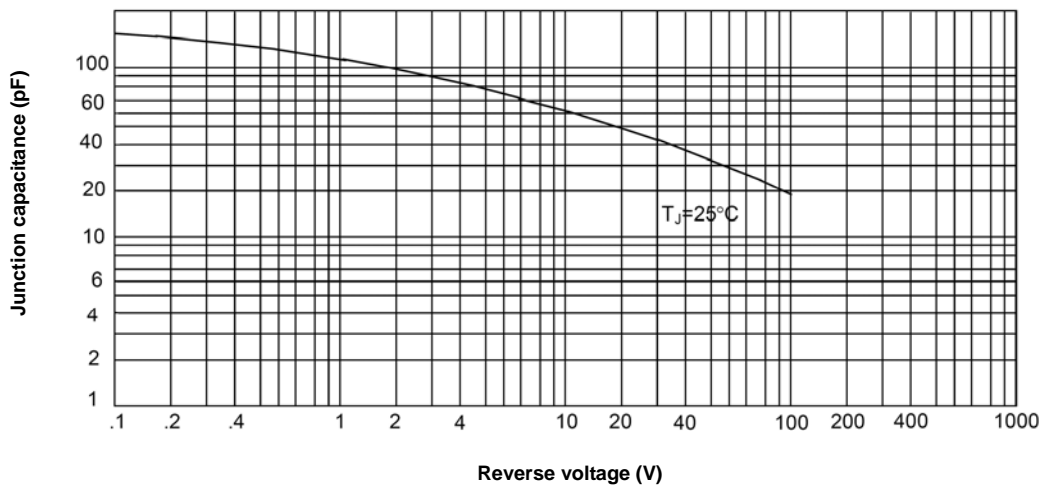
Figure 3. Junction capacitance
