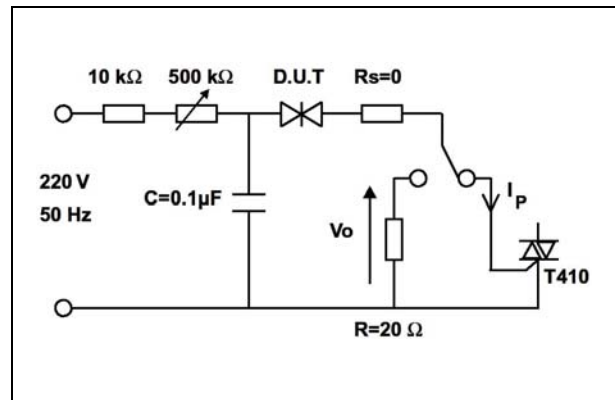
Diagram 2. Test circuit
