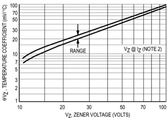
Figure 3. Temperature coefficients
